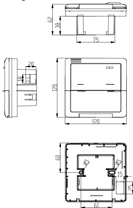
Fig.7.1 Installation Dimensions Diagram
