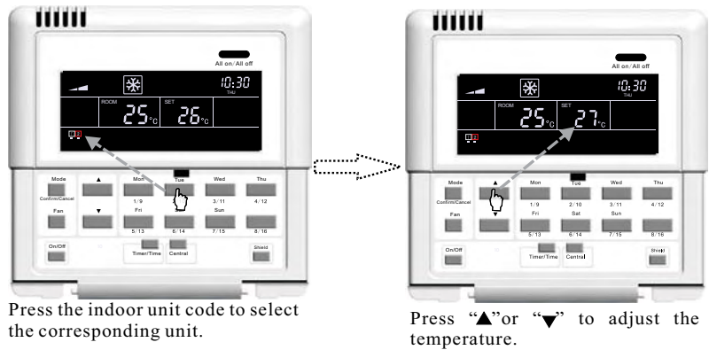
Fig. 5.2 Temperature Control under the Single Control
