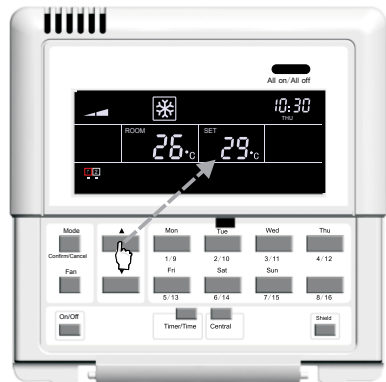
Fig.5.6 Temperature Adjustment
