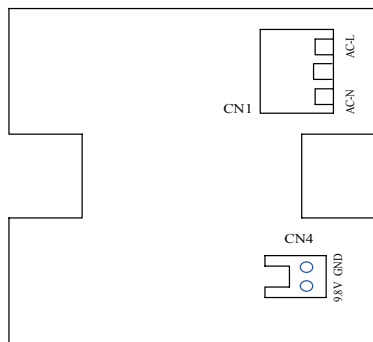
Fig.7.3 Interfaces of the Power Supply Module Board
