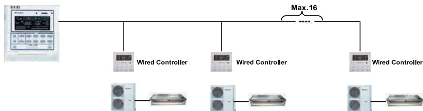
Fig.1.1 Unit Connection Diagram
