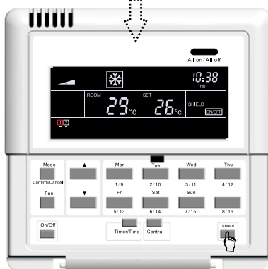
Fig.5.15 “ON/OFF” Shield under the Single Control
