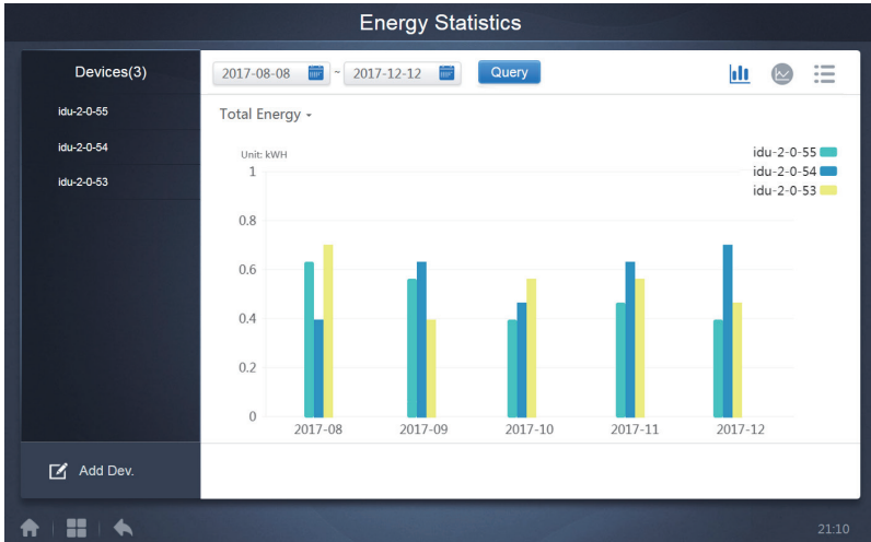
Histogram
