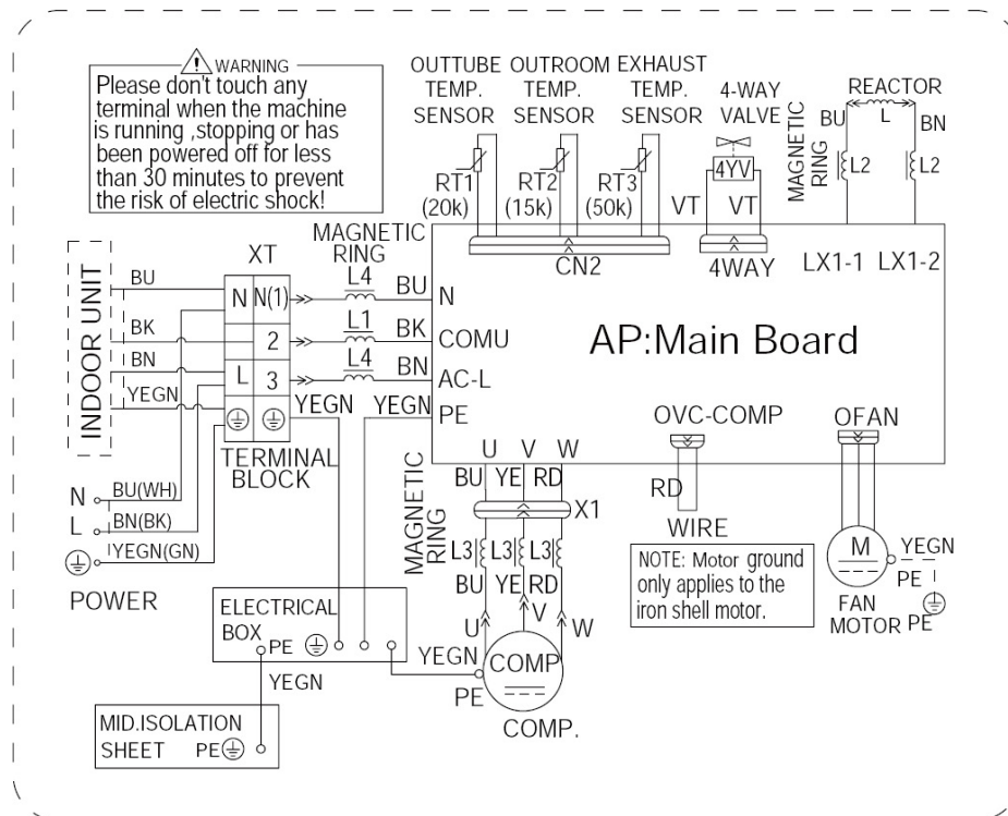
ASH-09AIR / ASH-12AIR outdoor unit
